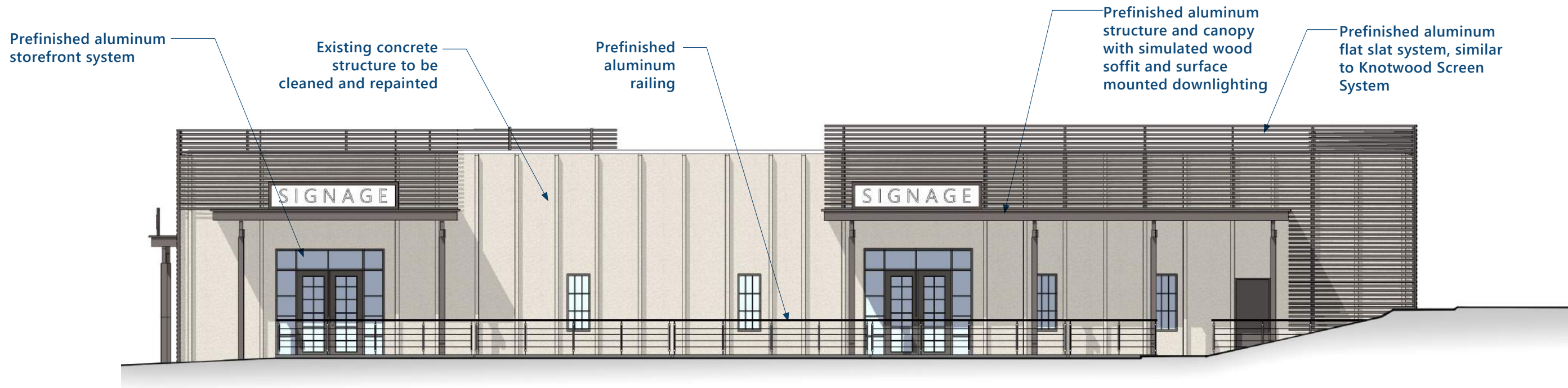
South Elevation
